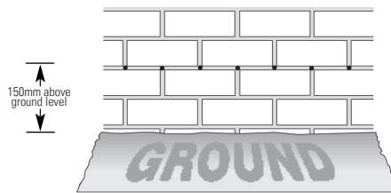
Figure 9: Drilling pattern for Stretching Bond
