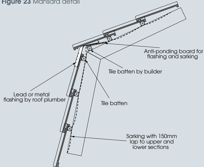
Figure 23 Mansard detail
