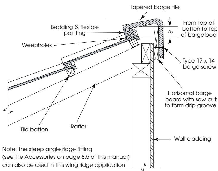
Figure 48 Steep pitch detail
