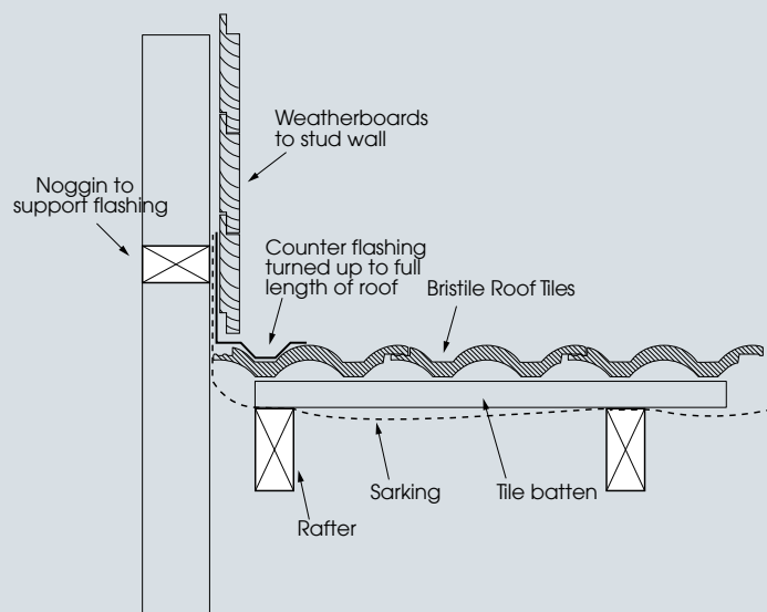
Figure 10 Flashing at side abutment
