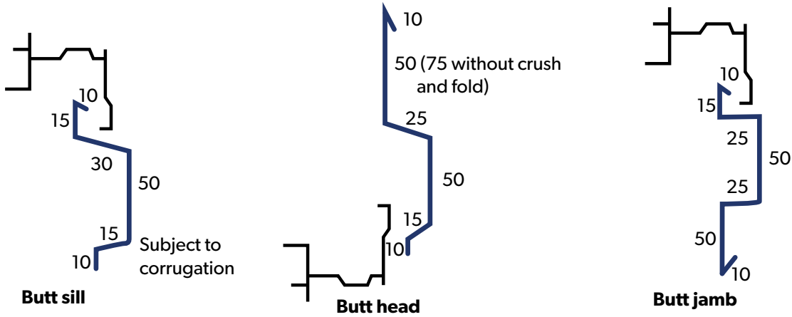
Figure 4.15.1 Butt window flashings (underlay is omitted for clarity)
