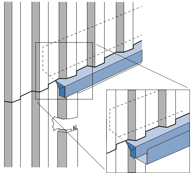
Figure 4.10.1 Flashings for vertical cladding
