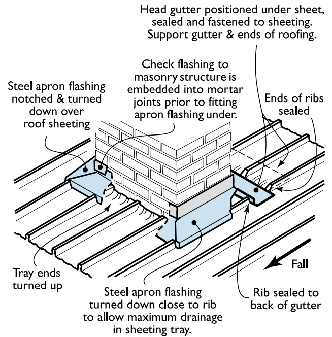
Figure 3.12.1 Flashing method 1: Head gutter
