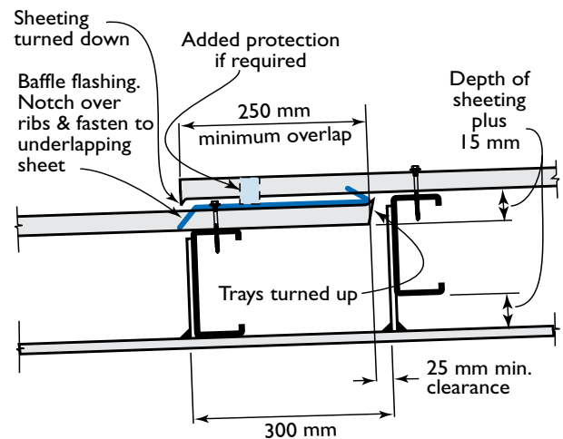
Figure 3.14.1 Expansion joint detail
