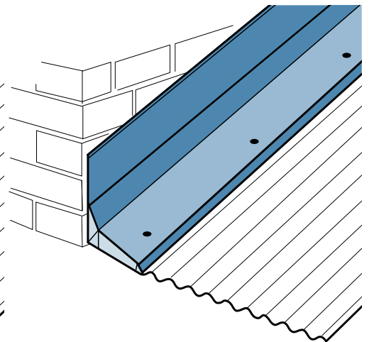
Figure 3.2.5 Angled apron 110°
