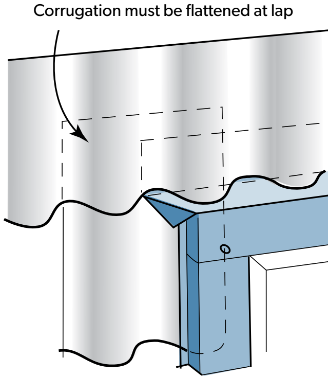
Figure 4.16.1 Head flashing for vertical cladding
