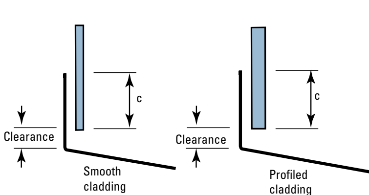
Figure 3.1.2 Vertical apron
