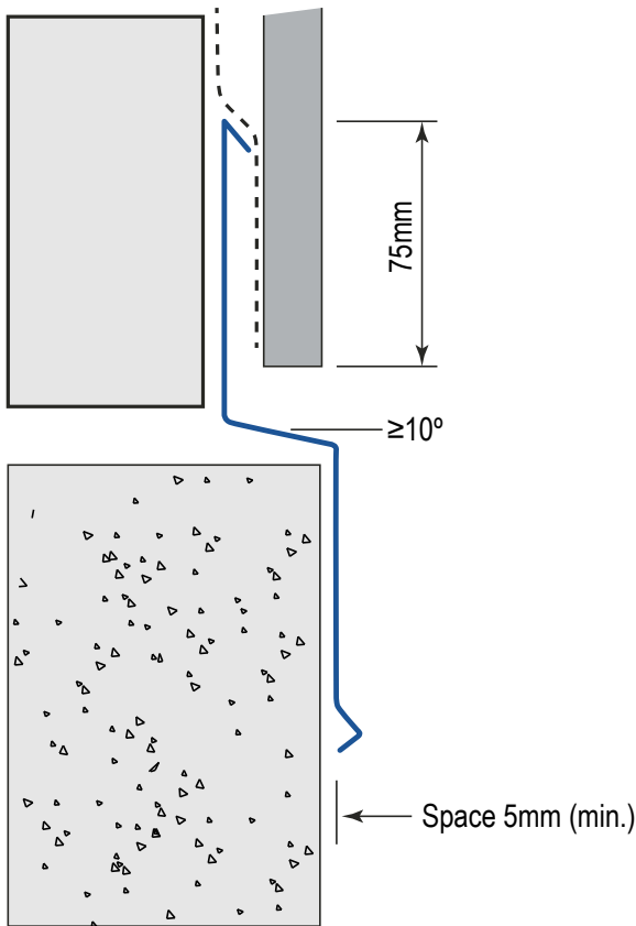
Figure 4.10.2 Flashings for vertical cladding
