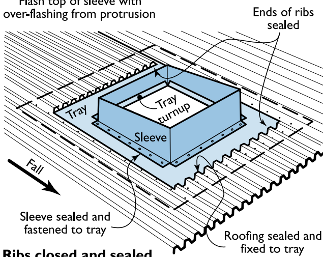
Ribs closed and sealed
