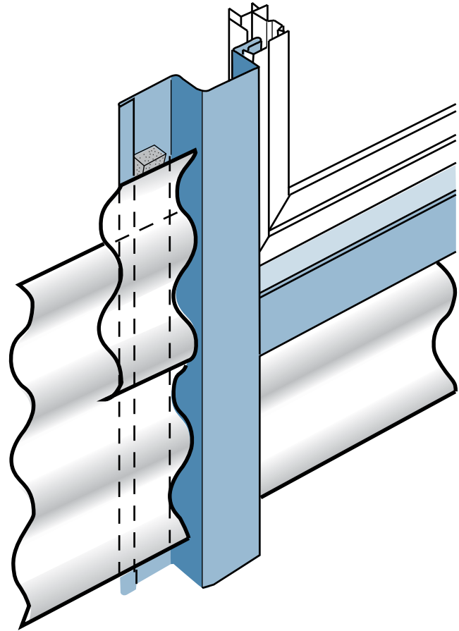
Figure 4.17.1 Alternative flashing designs
