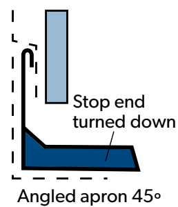
Figure 3.2.2 Angle diverter
