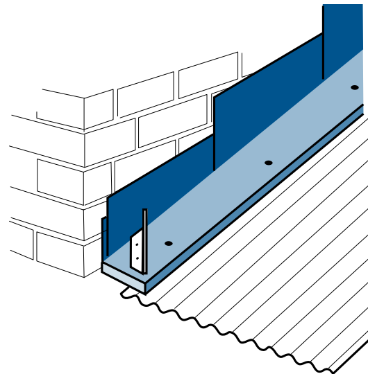
Figure 3.2.2 Angle diverter
