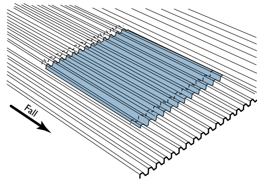
Type A Under soaker
