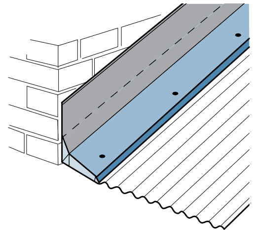
Figure 3.2.6 Two piece apron
