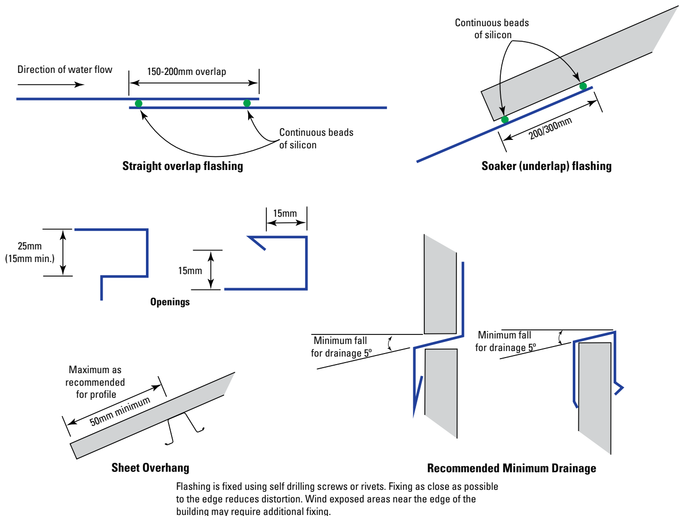
Figure 4.1.1 Types of flashing laps
