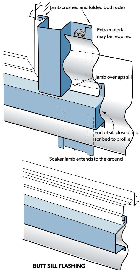
Figure 4.15.3 Butt window sill flashing
