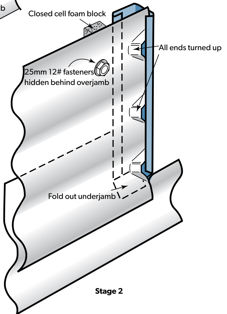
Figure 4.14.1 Flush window flashings
